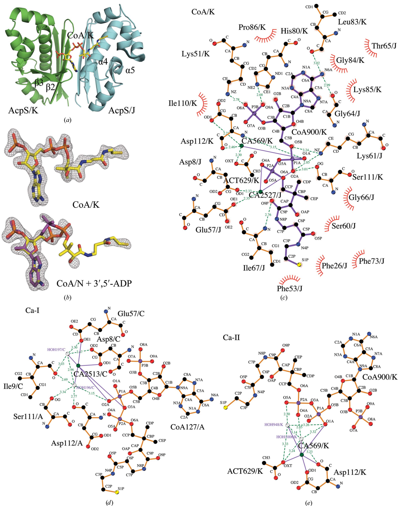
Figure 3 The structure of the binary CoA–Acp S Vc complex. (a) Interaction of CoA/K at the interface of the AcpS/K and AcpS/J protein molecules of the AcpS Vc /J/K/L trimer. CoA is colored according to its atoms: C, light yellow; N, blue; O, red; P, orange; S, dark yellow. (b) Examples of CoA molecules with well defined (CoA/K) and poorly defined (CoA/N) electron densities. The 2F_o - F_c maps are contoured at 1.0\sigma . The modeled 3',5'-ADP molecule at the CoA/N binding site is shown as purple sticks. (c) Coordination of CoA/K. (d) and (e) show the two calcium-binding sites, Ca-I and Ca-II. The coordination of CA2513/C in (d) is equivalent to that of CA2527/J in (e).
